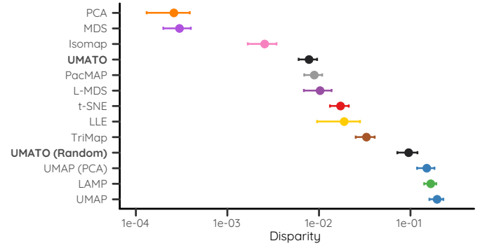
Fig. 7. The stability of UMATO and baseline techniques against subsampling (Section 4.3.1). The smaller the disparity is, the more stable the corresponding DR technique is. Error bars depict 95% confidence intervals.
