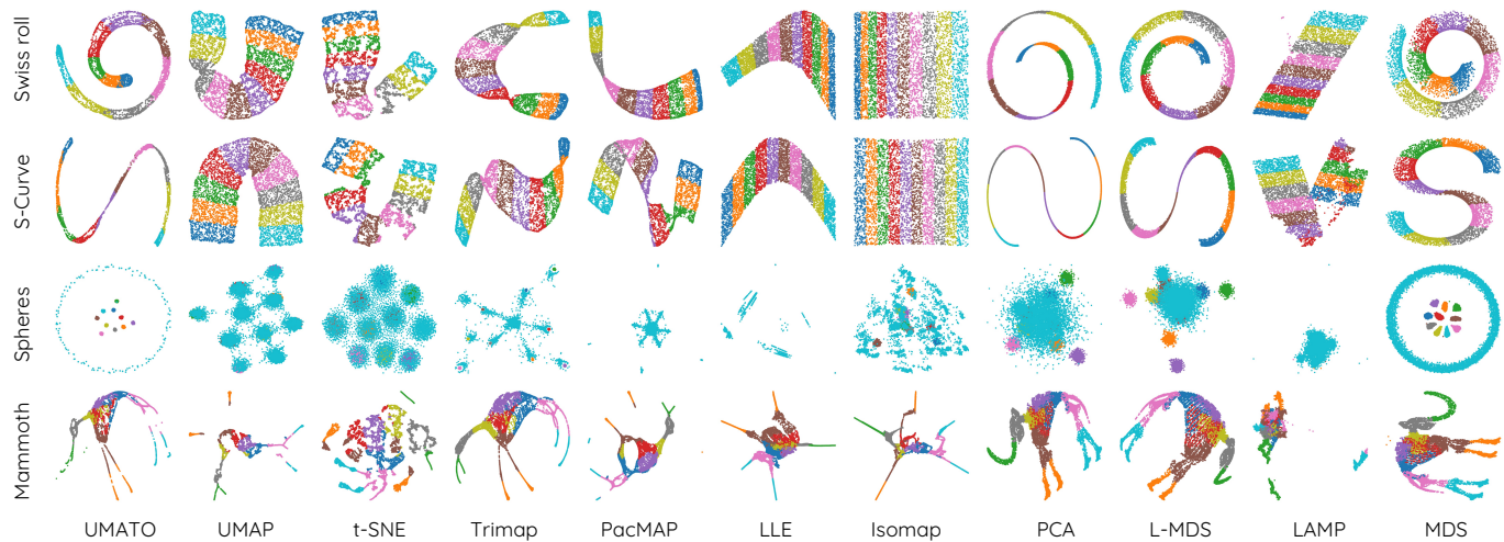
Fig. 9. The projections used in our qualitative experiment (Section 5). While UMATO succeeds in accurately depicting the original structure for all four datasets, competition techniques fail to do so.
